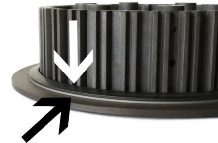
Jutter Spring on Inner Hub
