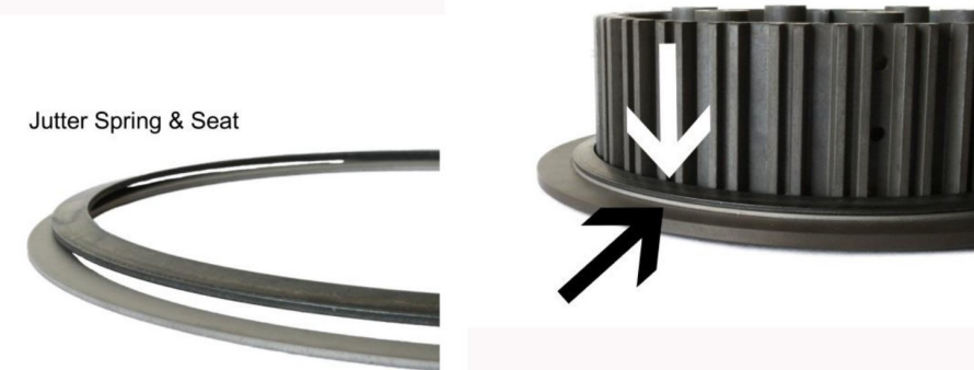
Jutter Spring on Inner Hub
